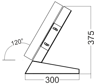
FABRICATED ARM WITH MONITOR SIDE VIEW
